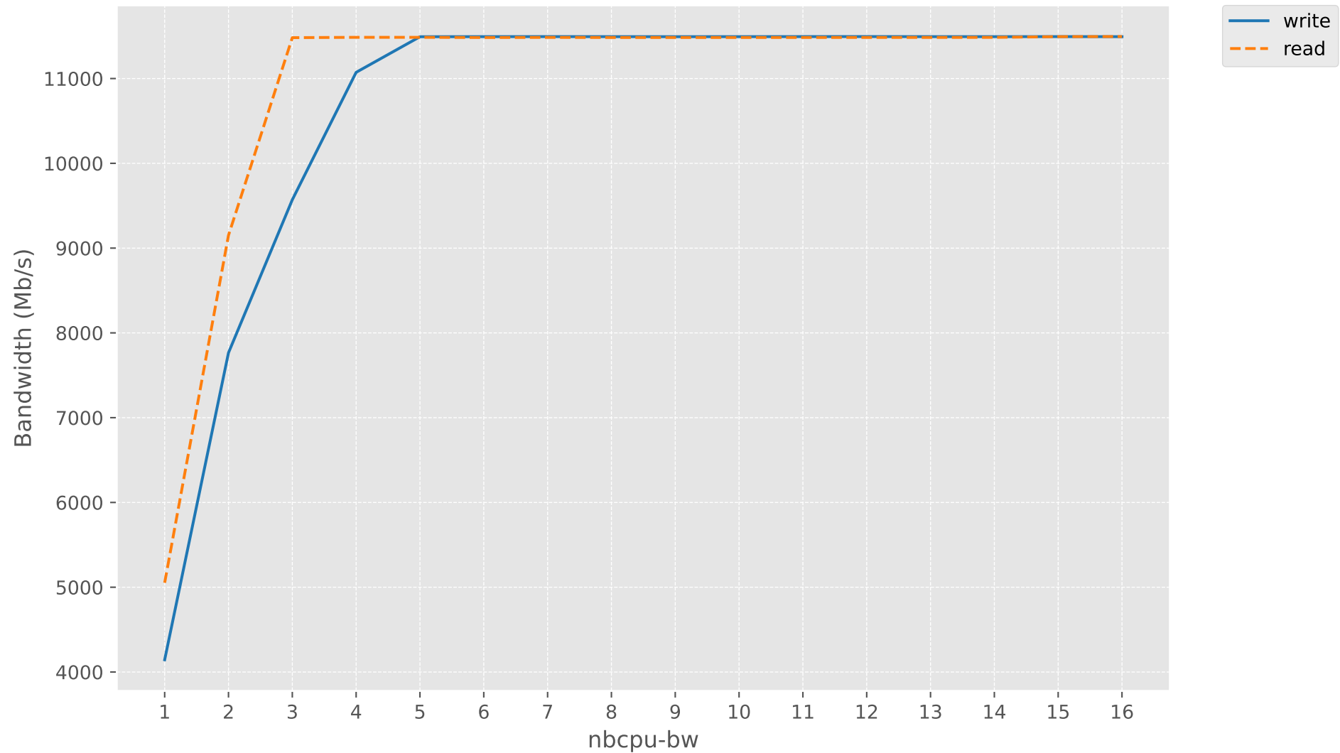
Bandwidth vs nbcpu-bw
